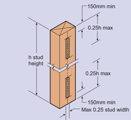
Safe drilling of studs
