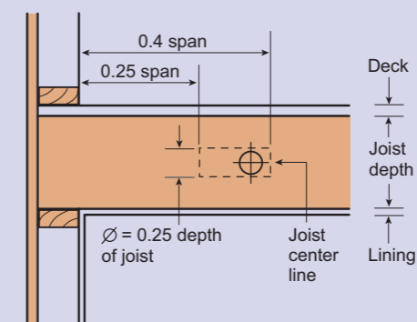
Safe drilling of joists
