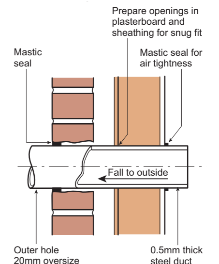
Fit the steel duct, making sure that it slopes downwards towards the outside
