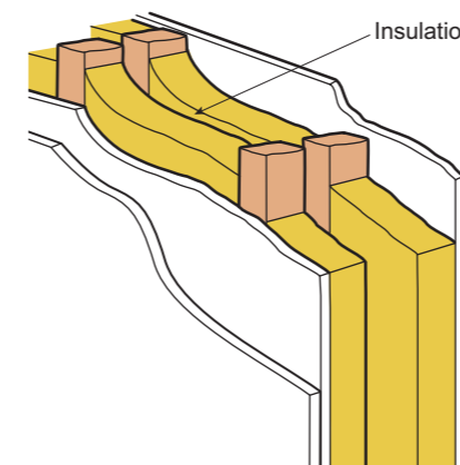
Party wall
