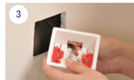
3 Pull the cable through the back of the box
