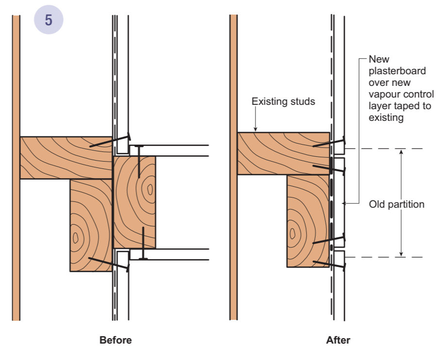
Wall/wall junction
