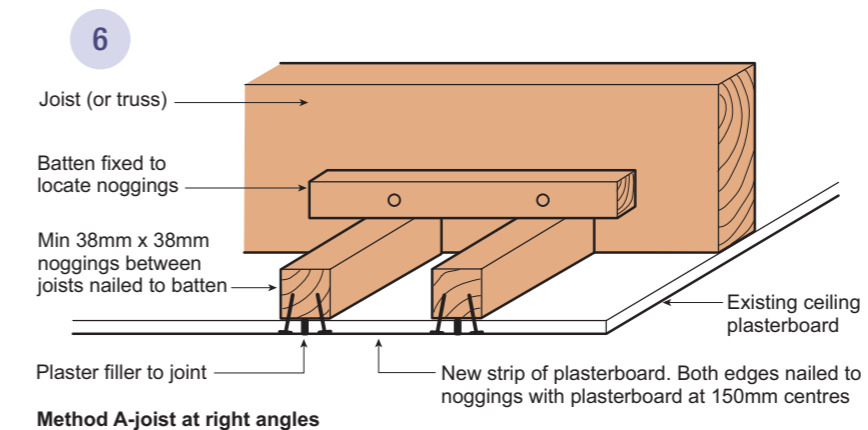
Method A-joist at right angles
