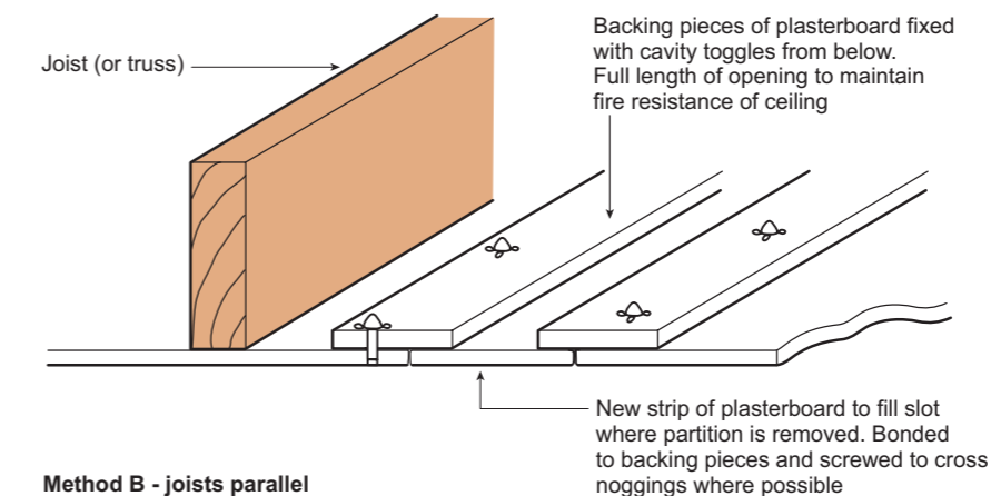
Wall/ceiling junction
