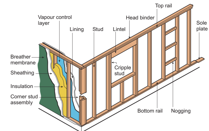
External wall frame
