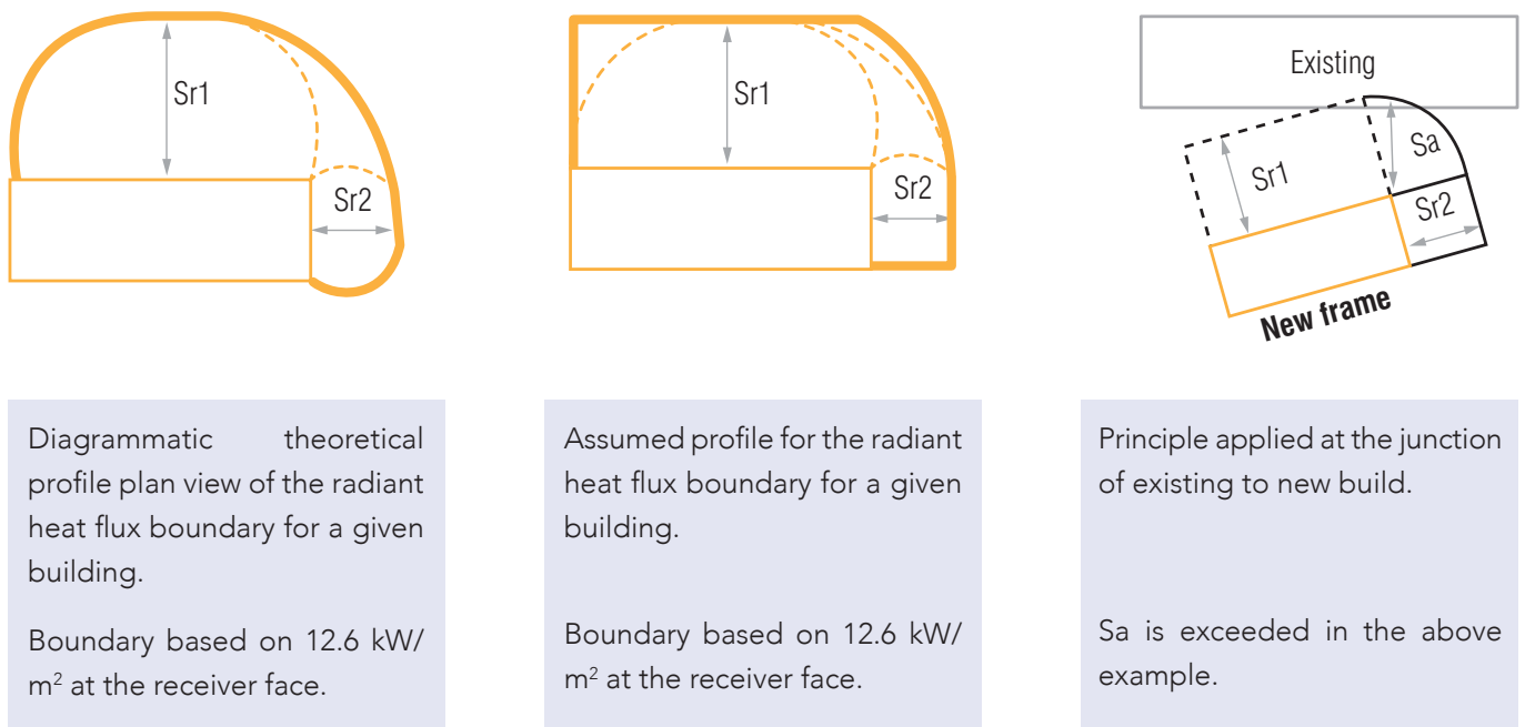
Figure 3.6: Buildings at angles to the emitter
