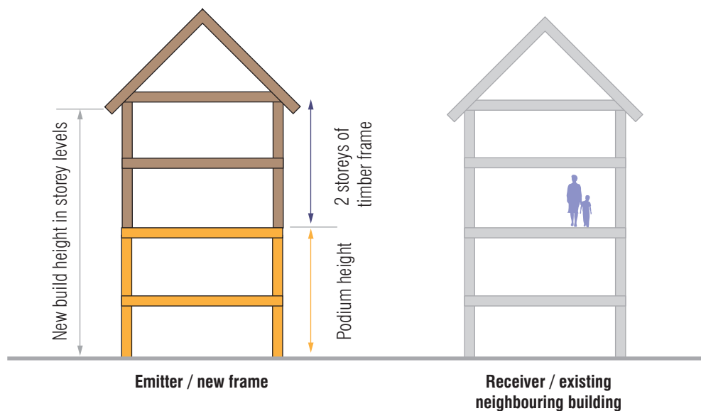
Figure 2.2: Emitter heights
