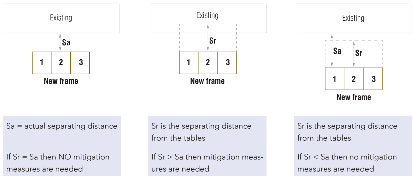
Figure 2.4: Comparing required distances to actual distances between buildings (Plan view)
