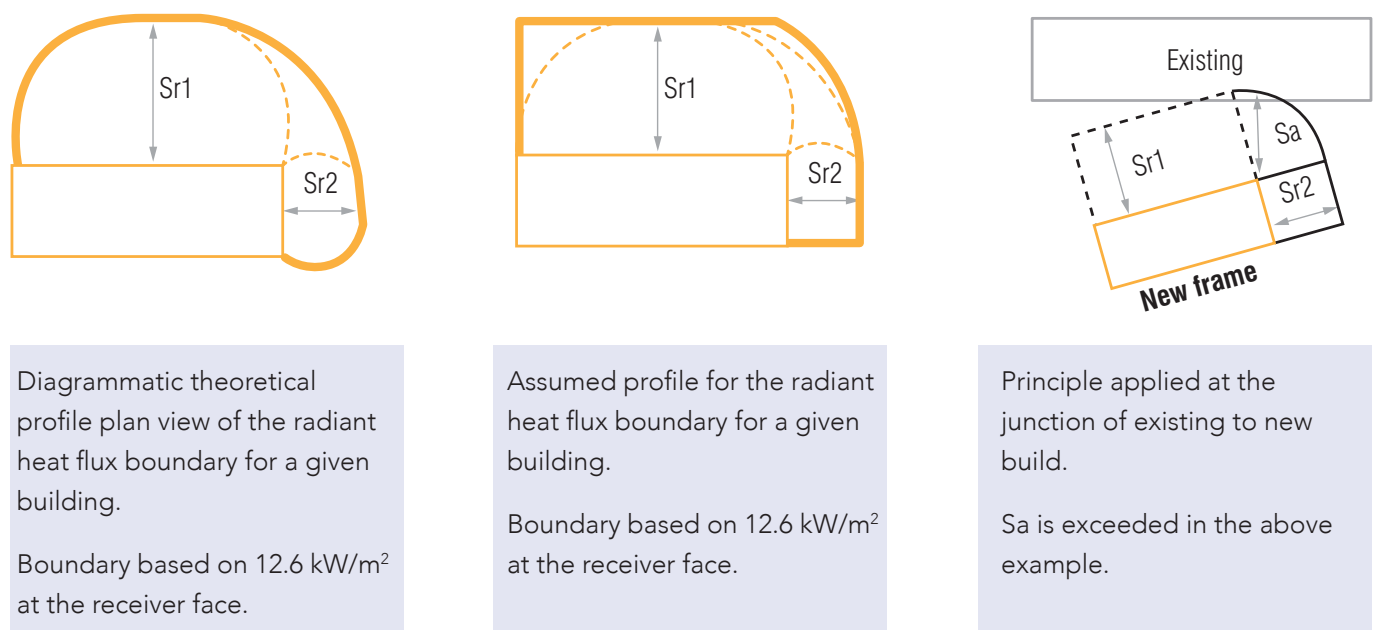
Figure 2.7: Buildings at angles to the emitter
