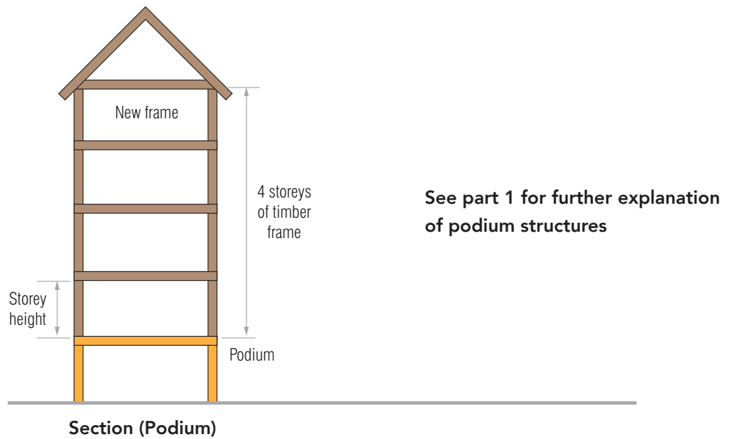
Figure 2.1: Example of storey heights and approach using podiums
