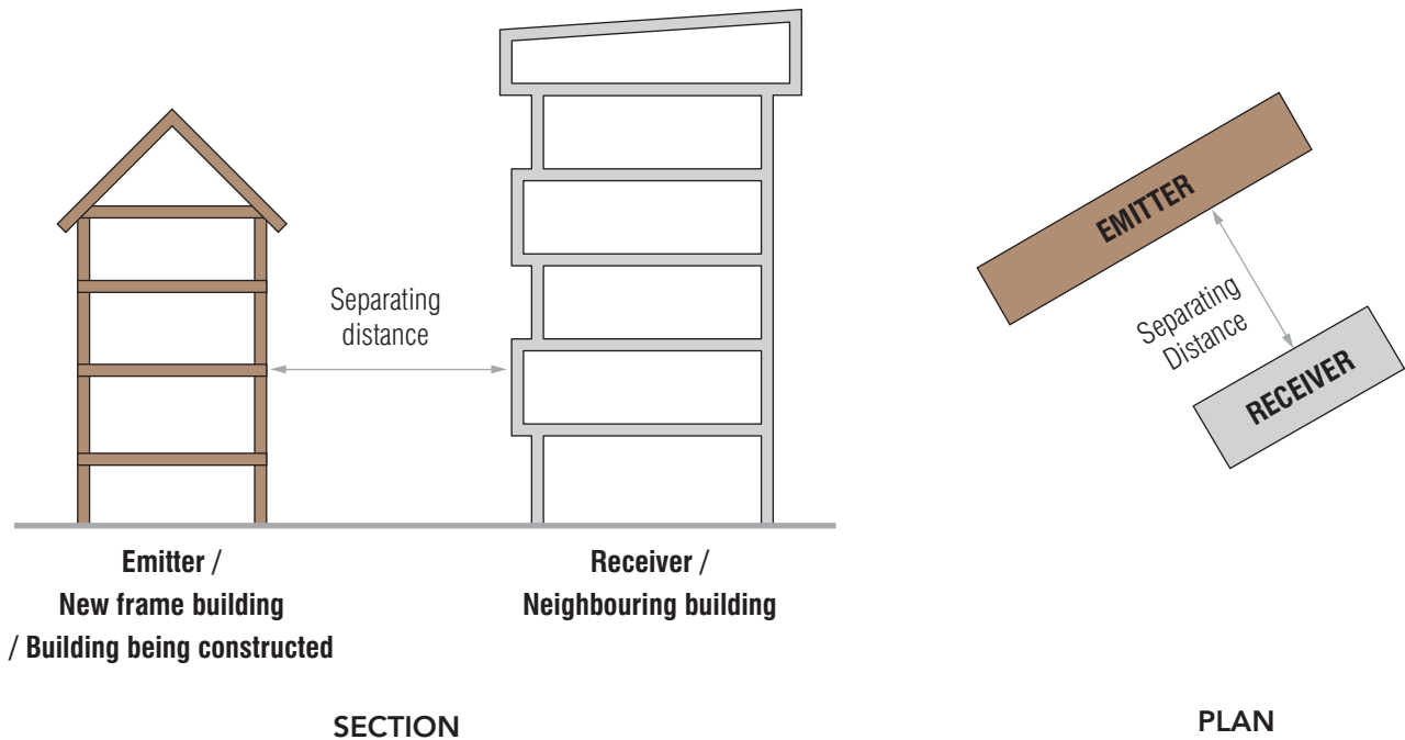
Figure 1.1: The separating distance is the nearest point between the emitter and receiver
